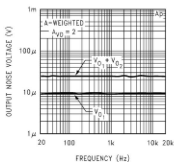
Noise Floor
